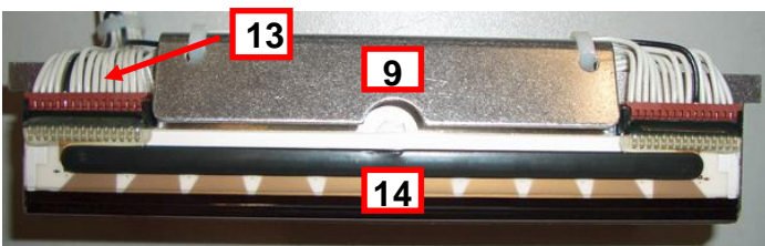
200 DPI Print Head (200L4)
