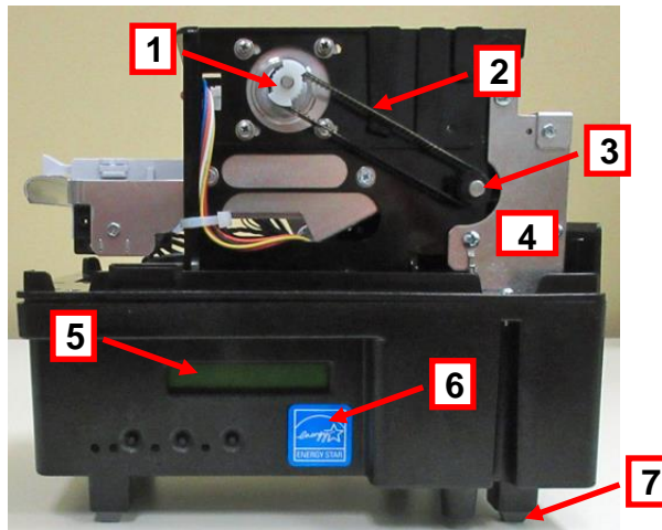
Above is Lemur with cutter and LCD display
